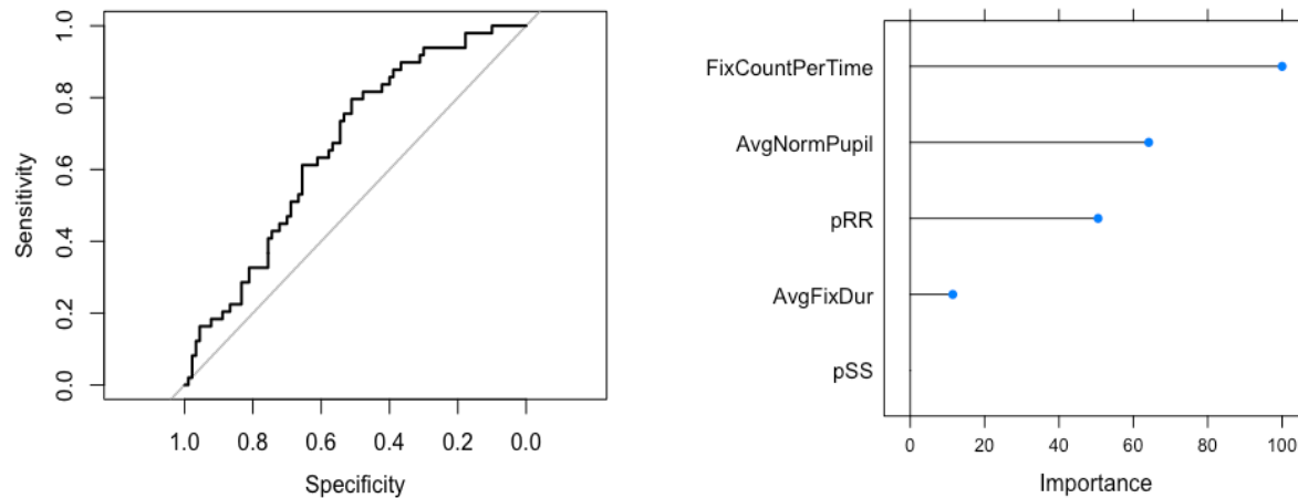
Figure 1. A ROC curve for FDA model and the relative importance of predictors in classification
